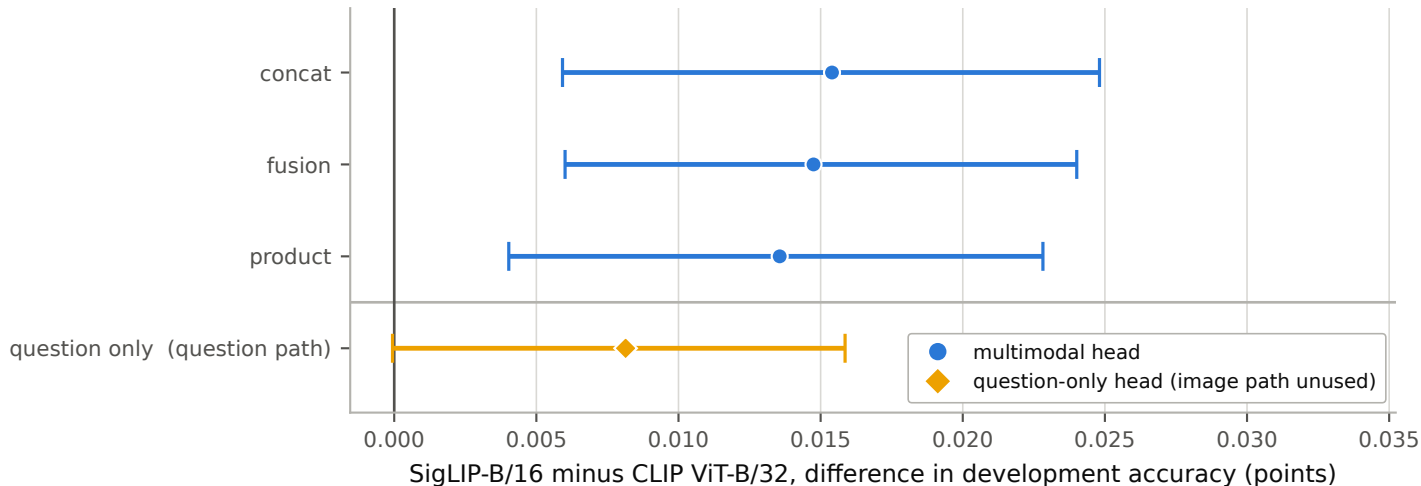
Representation-quality sensitivity at train_40k
